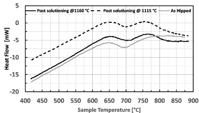
Figure 3. Differential Scanning Calorimetry (DSC) analysis for Astroloy in the as HIPped condition (gray line), after solutioning at 1160^\circ\text{C} (solid black line) and after solutioning at 1115^\circ\text{C} (dotted black line).
