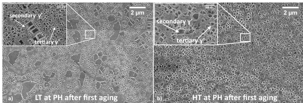
Figure 5. LT sample after aging at 760 °C for 8 h (a); HT sample aged at 760 °C for 8 h (b).
