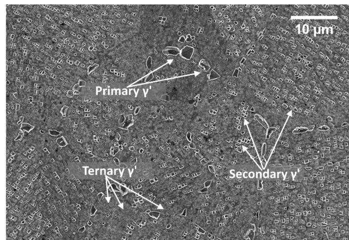
Figure 2. Generic micrograph showing the three \gamma' categories, i.e., primary, secondary and ternary.
