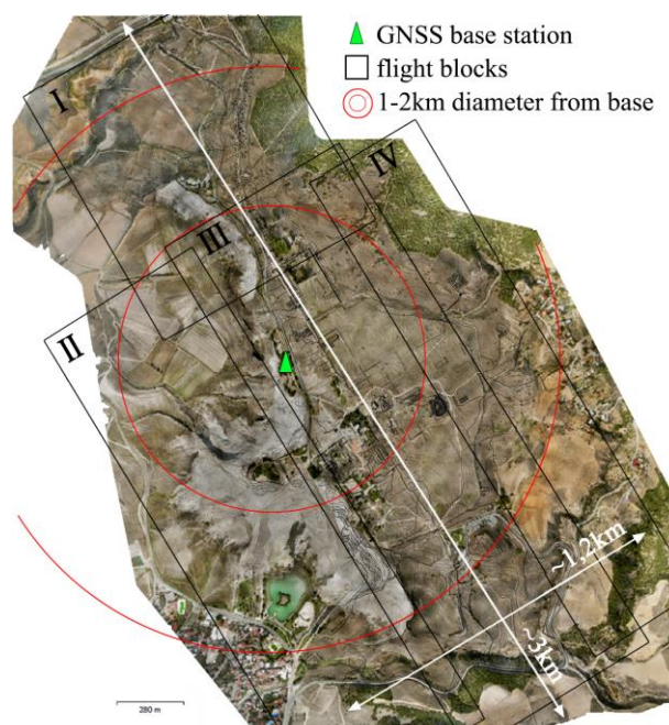
Figure 4. The resulting orthoimage of the site with indication of: the 4 flight blocks; the main extension dimensions and the GNSS base station position used for RTK/PPK positioning and its range of up to 1 km.
