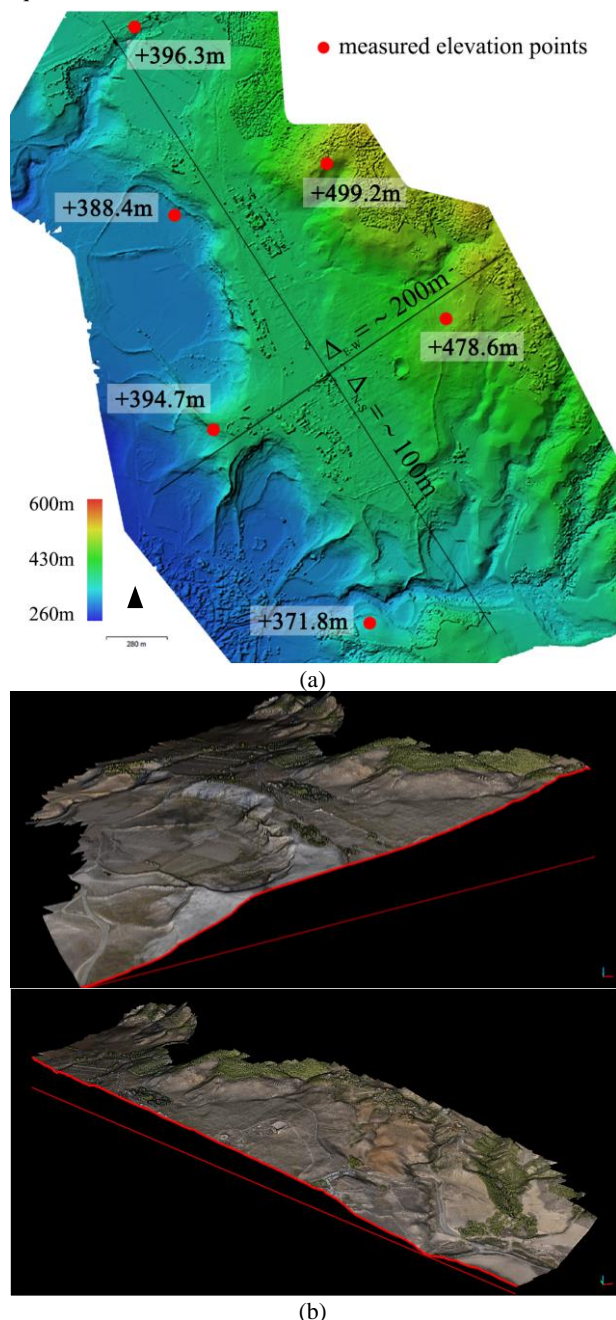
Figure 3. (a) The morphological characterization of the site with large differences in height towards the limestone hill, according the two main longitudinal and transverse section, reported in (b).
