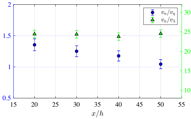
FIG. 4. Ratio of the characteristic TNTI speed \bar{v}_n normalized by the Kolmogorov v_\eta (full circles and left vertical axis) and by the Taylor velocity v_\lambda (full triangles and right vertical axis). Error bars indicate 7% of the measured value.
