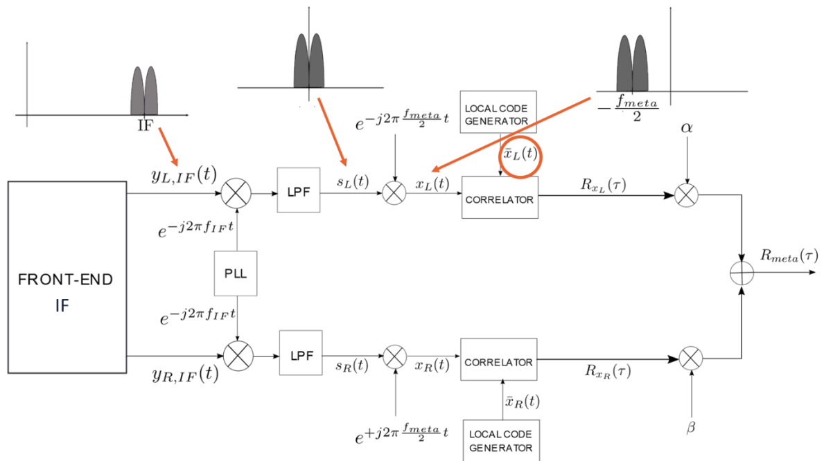
Figure 6. Open-loop scheme for virtual wide-band meta-signal processing.
