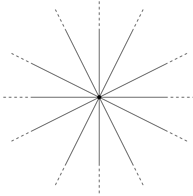
FIGURE 2. Example of infinite N -star graph ( N = 12 ).
