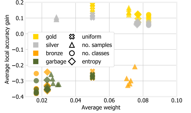
Fig. 4. Relationship between the weight assigned to local models and the local accuracy gain for different categories of nodes (identified by the color of markers), under different model-weighting strategies (identified by the shape of markers). Correlation coefficients for the “uniform”, “no. samples”, “no. classes” and “entropy” strategies are, respectively, 0, 0.07, 0.98 and 0.99.
