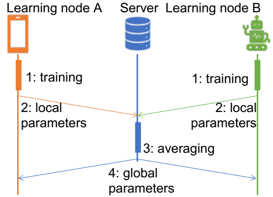
Fig. 1. Main steps of each iteration of the federated learning paradigm: learning nodes train their local model (1) and send the local parameters to the server (2); the server performs a weighted averaging of the model (3) and sends the global parameters back to the learning nodes (4).
