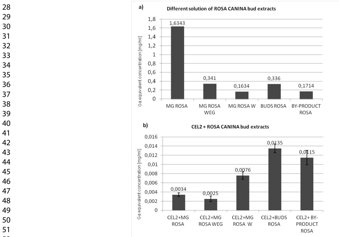
53 Figure 3: natural polyphenols amount expressed in GA equivalent for the uptake solutions (a) and for the sample (b)
