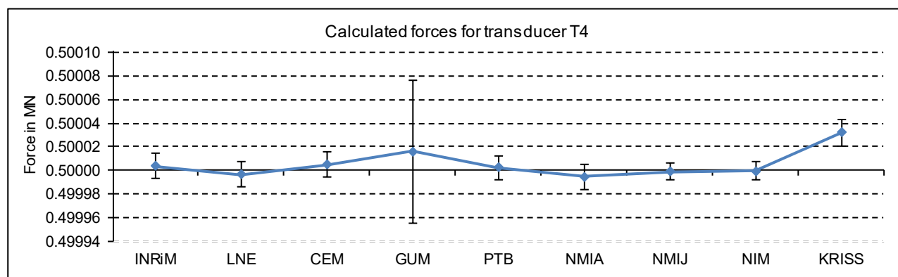
Figure 27: Calculated forces and expanded ( k = 2 ) uncertainties for transducer T4
