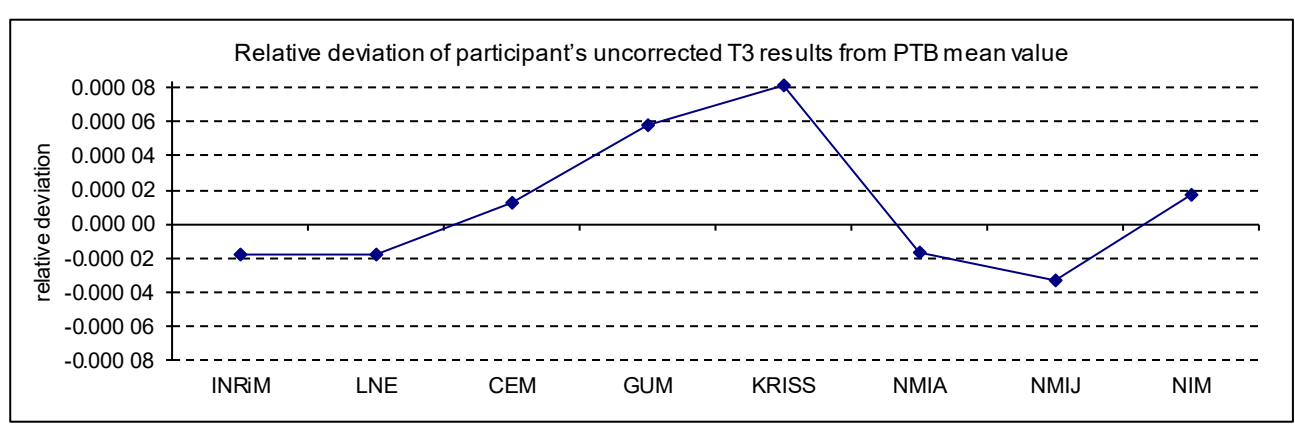
Figure 12: Relative deviation of participant's uncorrected results from PTB mean value (PTB01 to PTB13) for transducer T3
