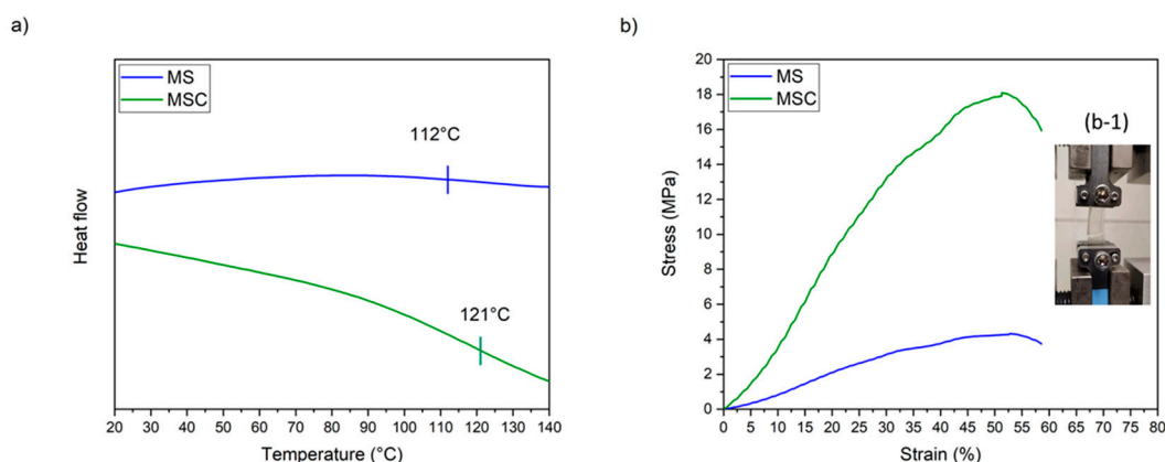
Figure 2. (a) DSC thermogram of MS and MSC; (b) Stress–strain curve of MS and MSC. (b-1) tensile fracture image.
