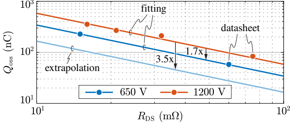
Fig. 6: Output capacitance charge Q_{\text{oss}} dependence on the drain-source resistance R_{\text{DS}} for the considered 650 V ( V_{\text{DS}} = 400\text{ V} ) and 1200 V ( V_{\text{DS}} = 800\text{ V} ) SiC MOSFETs from Wolfspeed [18]. The fitting curves assuming Q_{\text{oss}} \propto 1/R_{\text{DS}} are shown with straight lines. The 650 V characteristic obtained from analytical extrapolation of the performance of 1200 V devices according to traditional scaling laws [19] is illustrated for reference purposes, highlighting the significantly worse performance of real 650 V devices.
