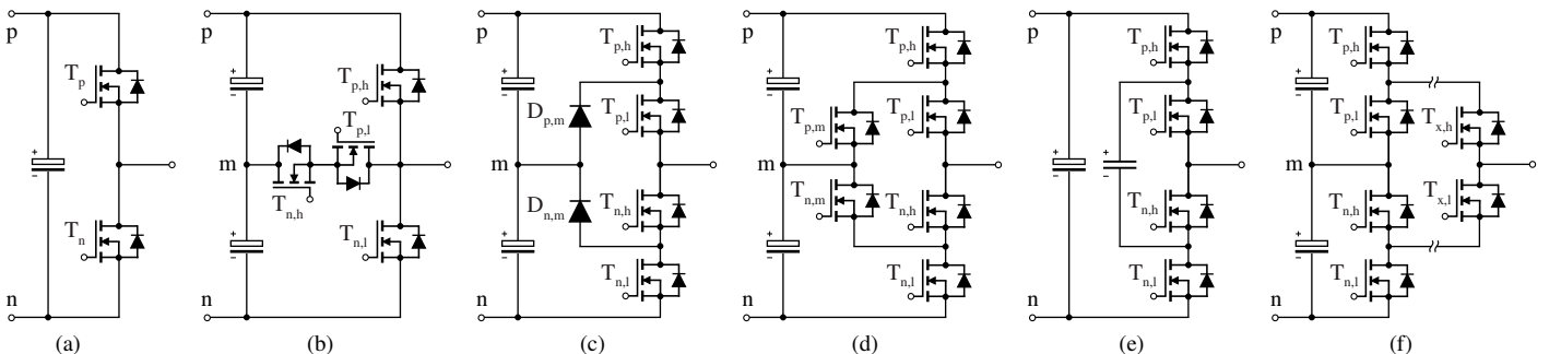
Fig. 1: Schematic of a single-phase bridge-leg of the (a) 2-level converter (2LC), (b) 3-level T-type converter (3LTTC), (c) 3-level neutral point clamped converter (3LNPCC), (d) 3-level active neutral point clamped converter (3LANPCC), (e) 3-level flying capacitor converter (3LFCC) and (f) 3-level sparse neutral point clamped converter (3LSNPCC). The 3LSNPCC bridge-leg includes the 3-L switching matrix and one 2-L inverter bridge-leg [9].
