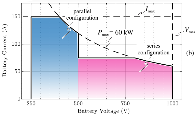
Fig. 4. Schematic overview of the proposed 60 kW modular DC fast charger (a). Highlight of the output voltage/current feasible operating region of the series/parallel reconfigurable DC/DC converter (b).
