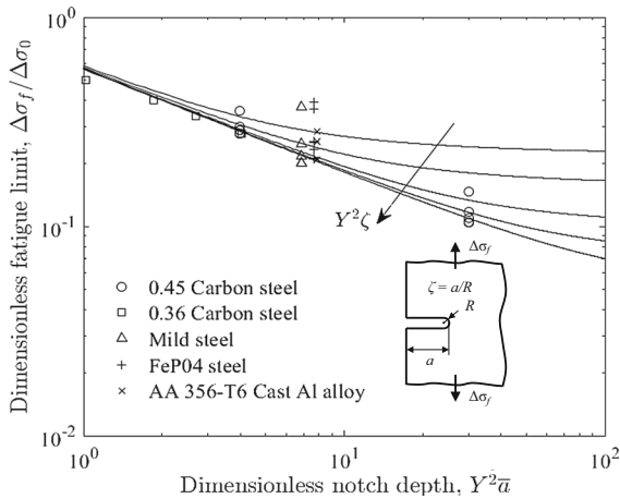
Fig. 7 U-notches: comparison between experimental data from (Harkegard 1981; Nisitani and Endo 1988; Lazzarin et al. 1997) and FFM predictions referring to different acutities; from the top to the bottom curves refer to Y^2 \zeta = 5, 10, 25, 50 and 100
