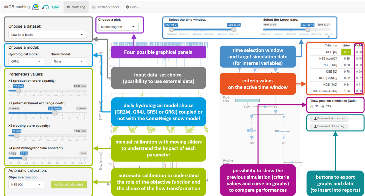
Figure B1. Graphical user interface of airGR using the airGRteaching package and describing the different functionalities.
