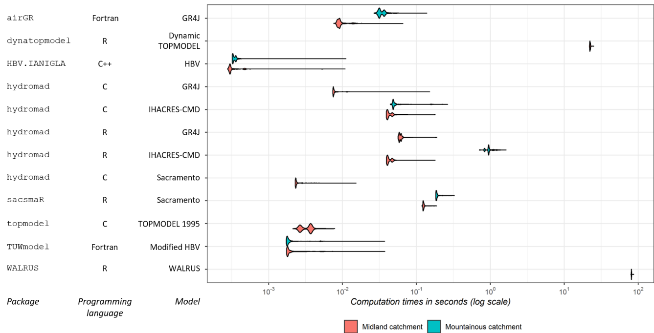
Figure 5. Computation times of the packages (time of one run estimated from 1000 runs using the same parameter set with the microbenchmark package). The models were run on a French catchment, the Meuse river in Saint-Mihiel, and a mountainous catchment, the Ubaye river at Lauzet-Ubaye, for a 10-year period at a daily time step. The related package functions were applied using the default settings, i.e. on a single spatial unit, except for dynatopmodel and topmodel . Runs on the mountainous catchment were performed only with the packages that integrate a snow function and use the default settings (i.e. five elevation bands for airGR and one for the other packages). hydromad includes an R version and a C version of GR4J and IHACRES-CMD. Data preprocessing and formatting are not taken into account in the estimation of computation times. Computer characteristics are as follows: RAM capacity – 8.00 GB; CPU – Intel i5-8250U 1.80 GHz; OS – Windows 10 (64 bit). R version 3.6.0 (64 bit) was used.
