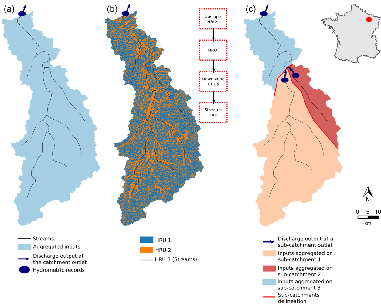
Figure 3. Illustration of the three possible spatial discretisations concerning the models contained in the selected packages for this study. From left to right are the lumped configuration, hydrological response units (HRUs) configuration and sub-catchments configuration. The catchment outline is from the Meuse river in Saint-Mihiel (France). The HRUs were generated using a function of the dynatopmodel package and are defined by the upslope area contribution based on the topographic index.
