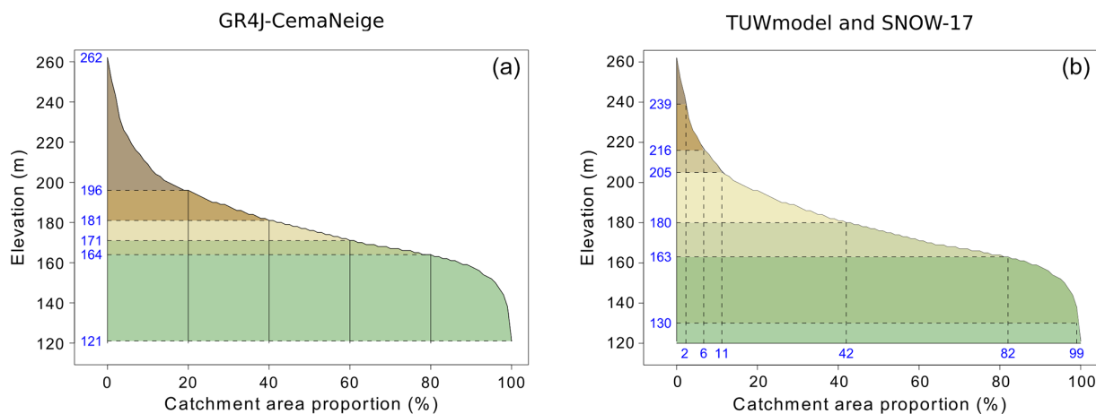
Figure 2. Example of GR4J-CemaNeige elevation zones (a) and TUWmodel/SNOW-17 elevation zones (b), with both following the hypsometric curve of the Couëtron river in Souday (France). Each colour indicates a different elevation zone.
