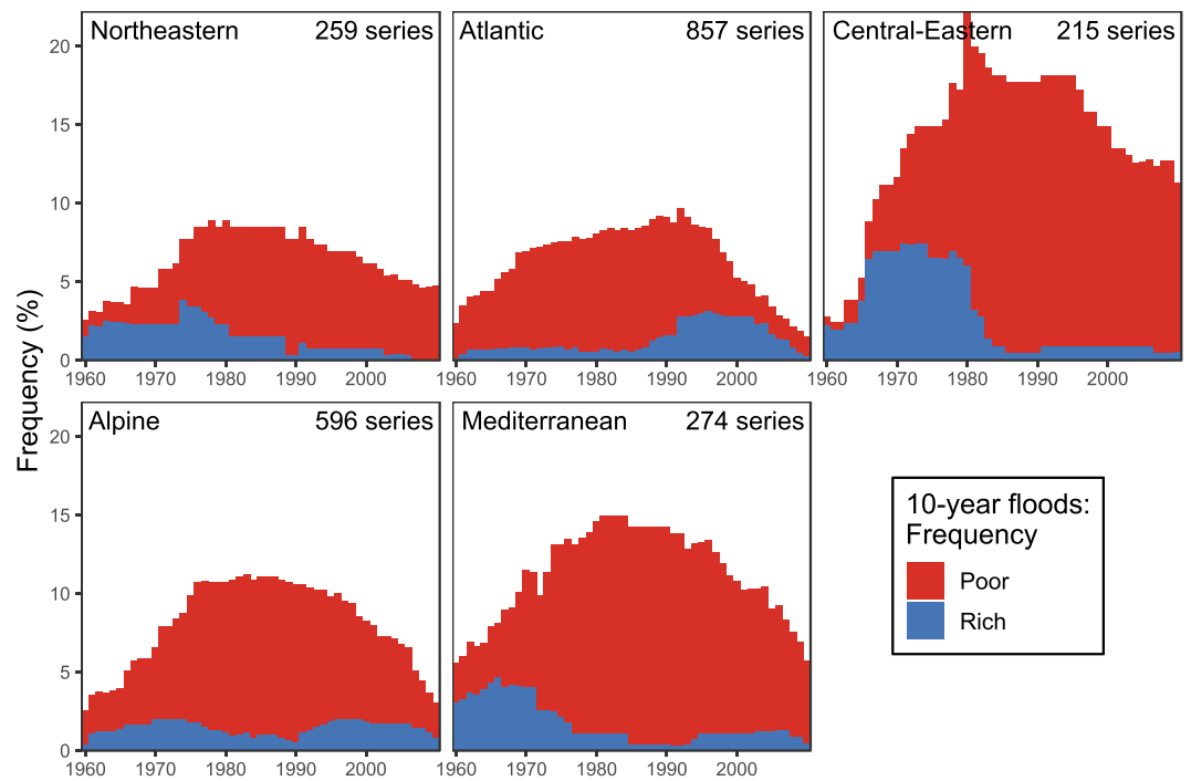
Figure A5. Frequency (%) of stations that exhibit a flood-rich or a flood-poor period in a given year as in Figure 4 but for a 10-year flood threshold.
