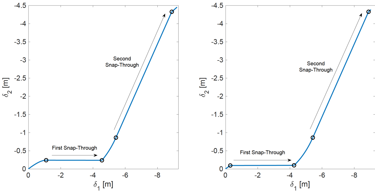
Figure 18: \delta_1 vs \delta_2 curves for increasing load: Case 1 (left graph) and Case 2 (right graph)
