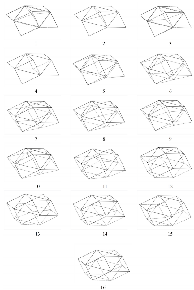
Figure 12: Sixteen-member structure displacements (Case 1 - \lambda_{up} = 13.0 )
