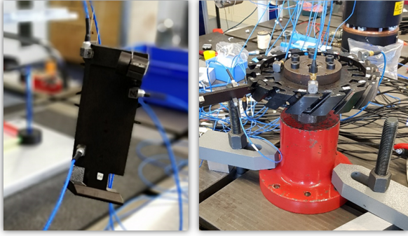
FIGURE 5. The measurement setup: the blade (left) hunged with rubber mounts and the disk (right) constrained at the center with a flange.
