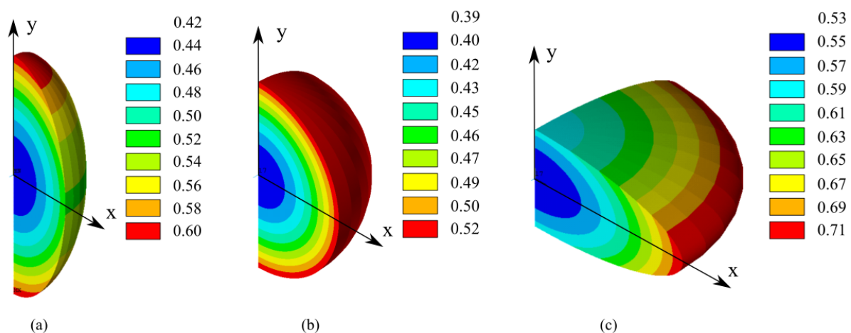
Figure 9. Normalized concentration distribution ( \bar{c} = c/c_{max} ) in sphere, \alpha = 1 (b) and in ellipsoids, \alpha = 0.5 (a) and \alpha = 3.5 (c). Chemical and mechanical properties are listed in Table 2: lithium flux is 1 \text{ A/m}^2 and simulation time is 1000 s.
