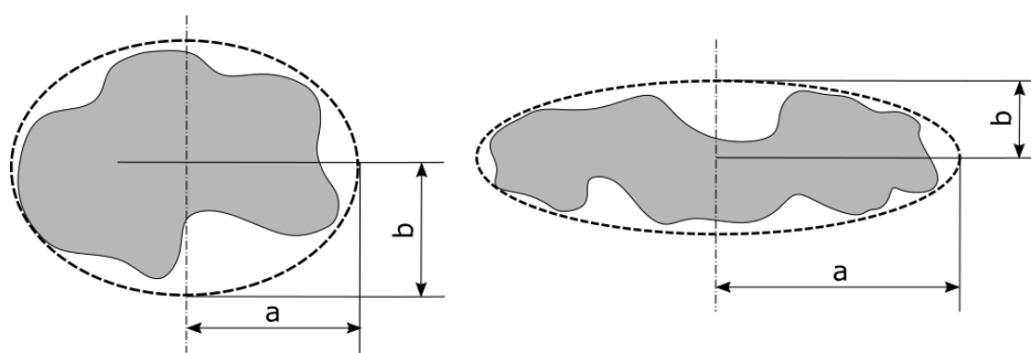
Figure 1. Sketch of a section of an hypothetical real particles in grey and the equivalent elliptical geometries in dashed line. Aspect ratio is defined as \alpha = a/b . Ellipsoid is constructed rotating one half of the section around its central vertical axis.
