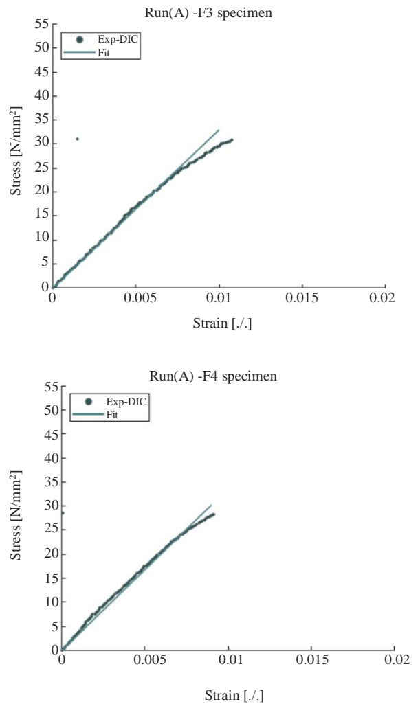
Fig. 10: Run(A): Free (F) specimens; tensile stress Vs. longitudinal strain curves; (a) Run(A)-F3; (b) Run(A)-F4
