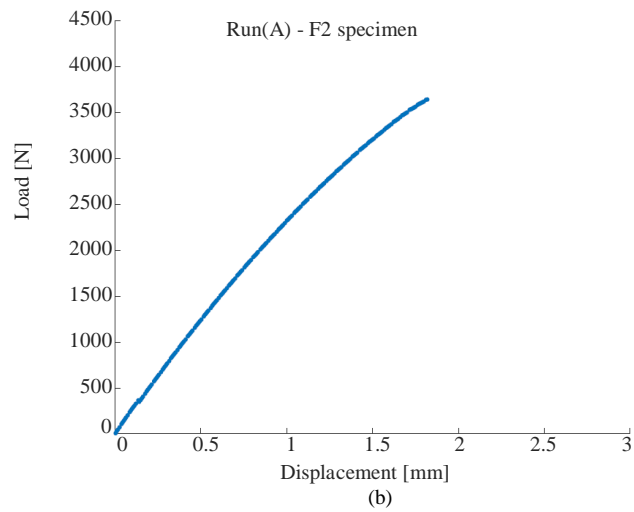
Fig. 2: Run(A): Free (F) specimens; tensile load Vs. longitudinal displacement curves; (a) Run(A) - F1; (b) Run(A) - F2
