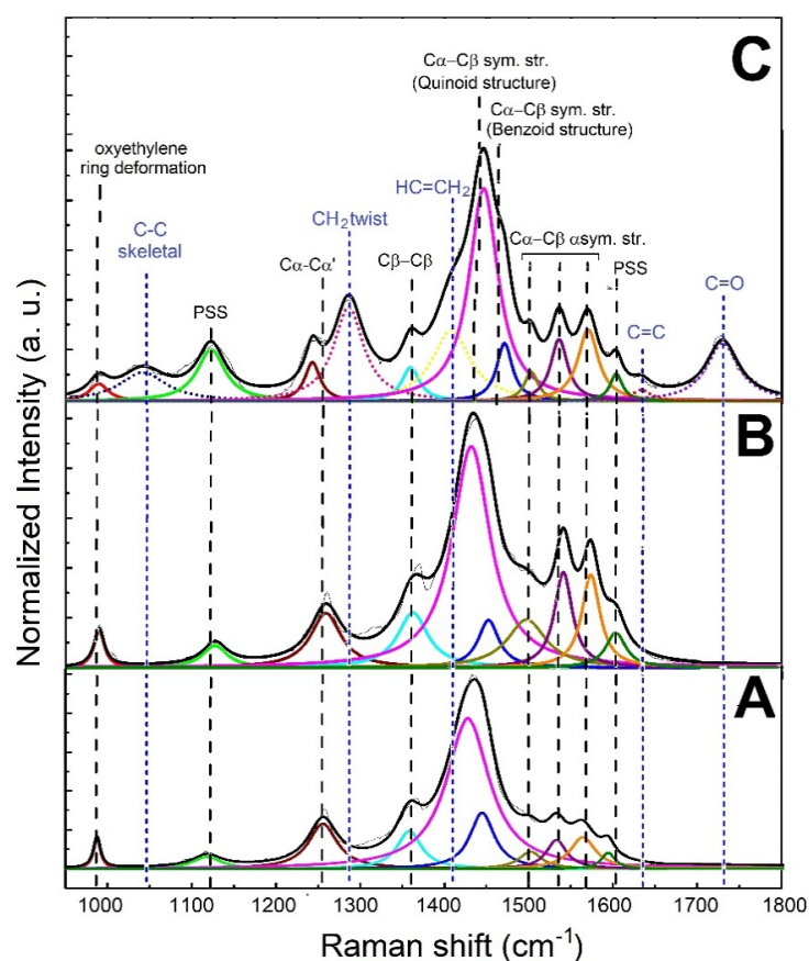
Figure 4. Raman spectra of (A) untreated PEDOT:PSS, (B) treated PEDOT:PSS and (C) printed PEGDA:PEDOT.
