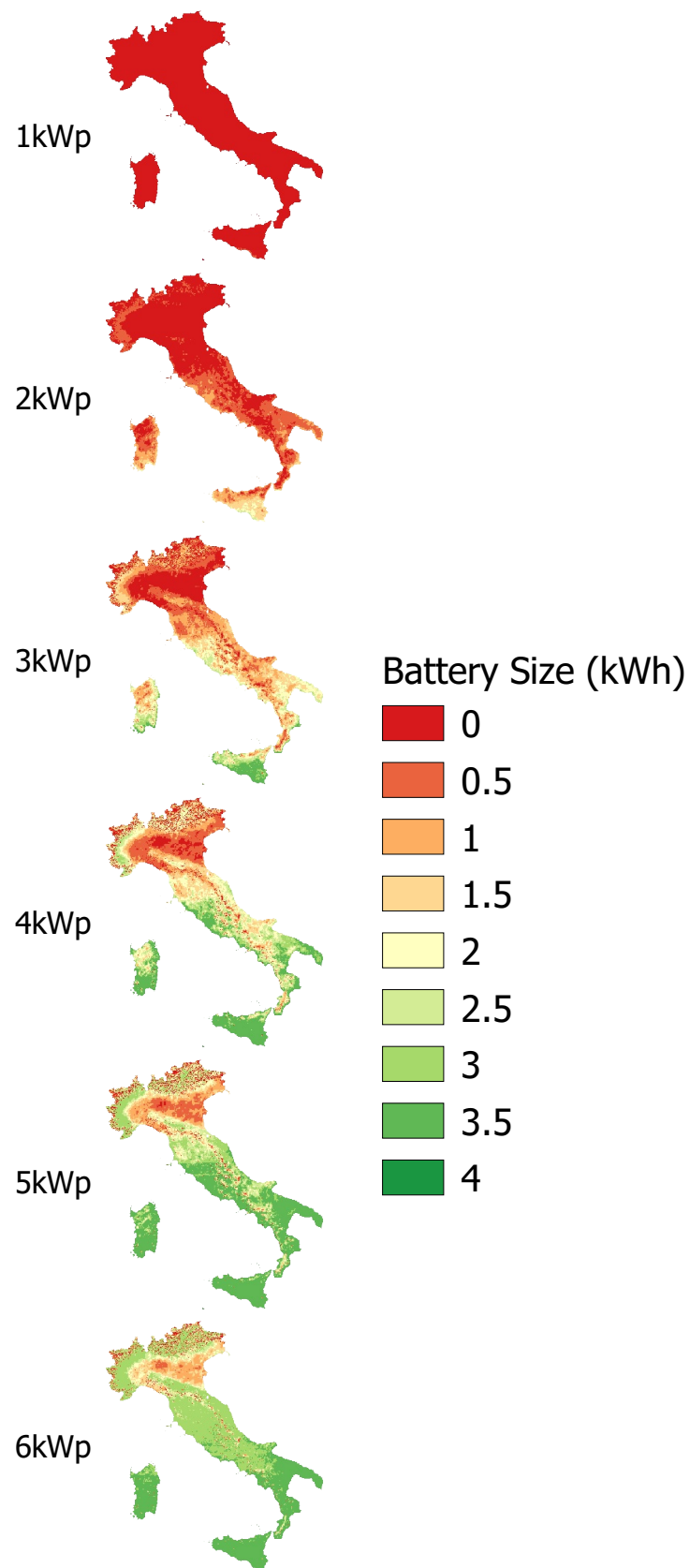
Figure A1. Battery size for E_L = 2700 kWh.
