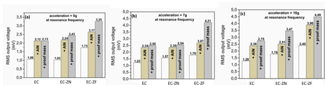
Figure 1. Root Mean Square output voltage values obtained by the different fabricated beams configurations at their resonance frequency for three acceleration values: (a) 5 g, (b) 7 g and (c) 10 g.
