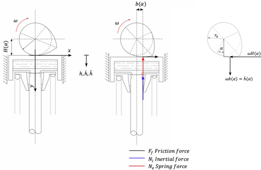
Figure 1. Schematization of the forces exerted at the cam-tappet interface.
