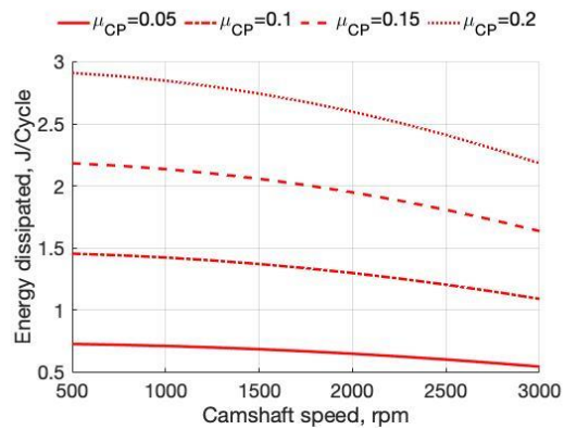
Figure 6. Friction dissipation trends for 1 cam in 1 cycle, parameterized for friction coefficient.
