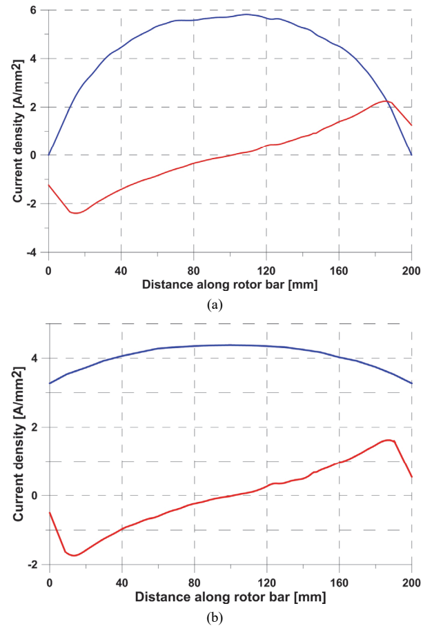
Fig. 4. Current density distributions at the upper surface of the bar carrying the maximum current (same conditions as Fig.3, contact resistance = 24\mu\Omega ): (a) on the path shown in Fig.3.a, (b) on a line parallel to the previous path positioned inside the bar at the distance \Delta h shown in Fig. 2 – Blue: component along bar, red: component perpendicular to the bar.
