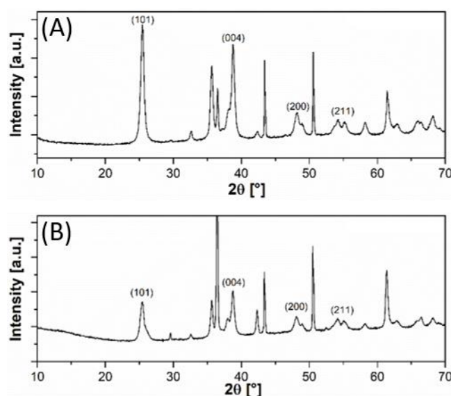
Figure 1 XRD patterns of electrodes obtained from (A) pristine and (B) 50 wt% PEG additivated \text{TiO}_2 pastes. Samples were deposited onto a Cu foil as a substrate and then annealed as described in the Experimental Section.
