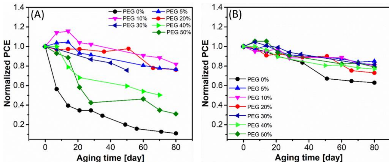
Figure 7 Long-term stability of aqueous DSSCs assembled with (A) liquid or (B) quasi-solid state electrolytes. Normalized efficiency for cells assembled with photoanodes obtained from different PEG-based pastes is shown. During aging, cells were stored under dark and at room temperature.
