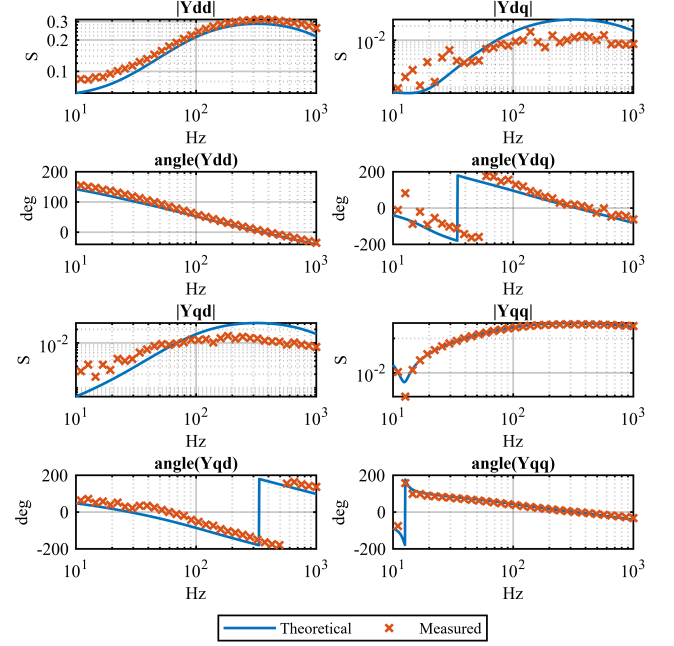
Fig. 6. Experimental results of the voltage injection method ( i_d^* = 10A, i_q^* = 0A ).
