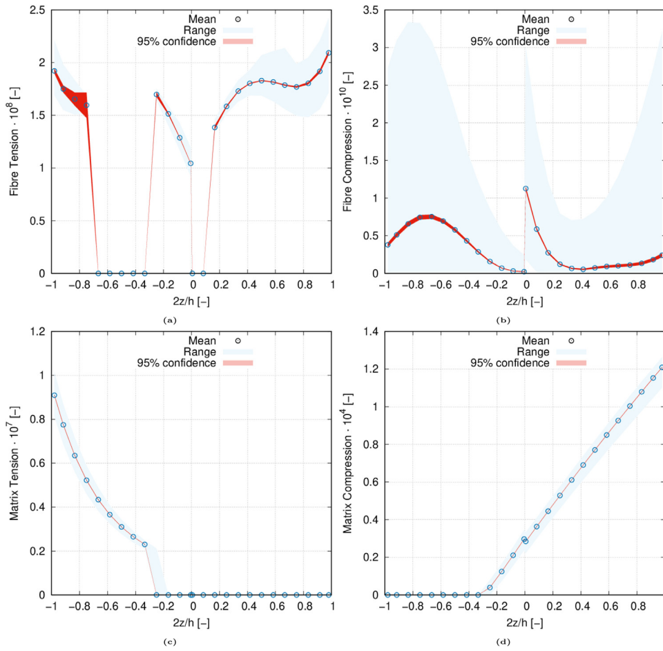
Fig. 11. Through-the-thickness failure index based on Hashin 3D, measured at point Q, for the pristine and flawed structure. The [ < 90, 45 >, < 0, 45 > ] plate is clamped in its four edges and a constant pressure Pz = -10 kPa is exerted at z = h/2 . Mean value, range and 95% confidence interval are displayed. The fibre misalignment field has a null mean and standard deviation equal to \sigma_\theta = 1.5^\circ .
