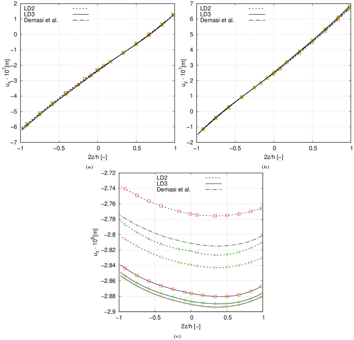
Fig. 6. Through-the-thickness displacement field, measured at point Q, for the different number mesh elements and element theory. 6×6 mesh \square , 8×8 mesh \triangle , 10×10 mesh \circ . LD2 and LD3 stand for quadratic and cubic element order. The [< 90, 45 >, < 0, 45 >] plate is clamped in its four edges and a constant pressure P_z = -10 kPa is exerted at z = h/2 .
