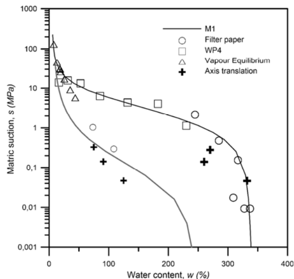
Fig. 6. Water retention of M1 samples: w - s .
