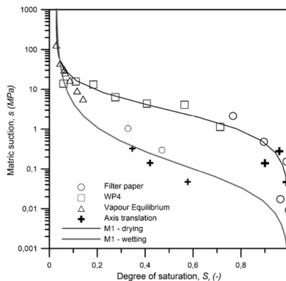
Fig. 5. Water retention of M1 samples: S_r - s .
