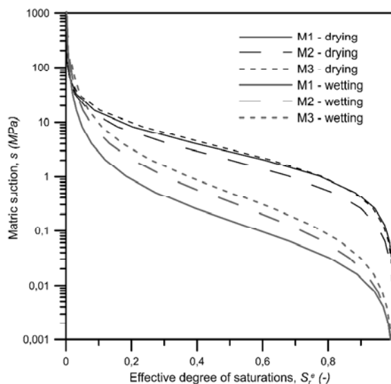
Fig. 7. S_r^e - s fits for the three mixtures.
