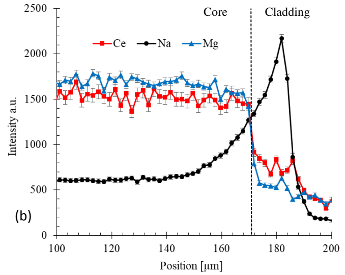
Figure 4. (a) EDS line scan across the entire cane where the core (Mg) and core/cladding (Si) components can be seen, and (b) spectra of the core-cladding interface for Mg, Ce, and Na.
