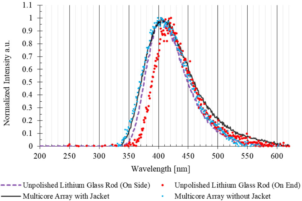
Figure 3. Radioluminescence spectra characteristic of \text{Ce}^{3+} activator emission for the unpolished ^6\text{Li} glass rod (unprocessed) and the multicore arrays (drawn into fibers) with and without outer jackets.
