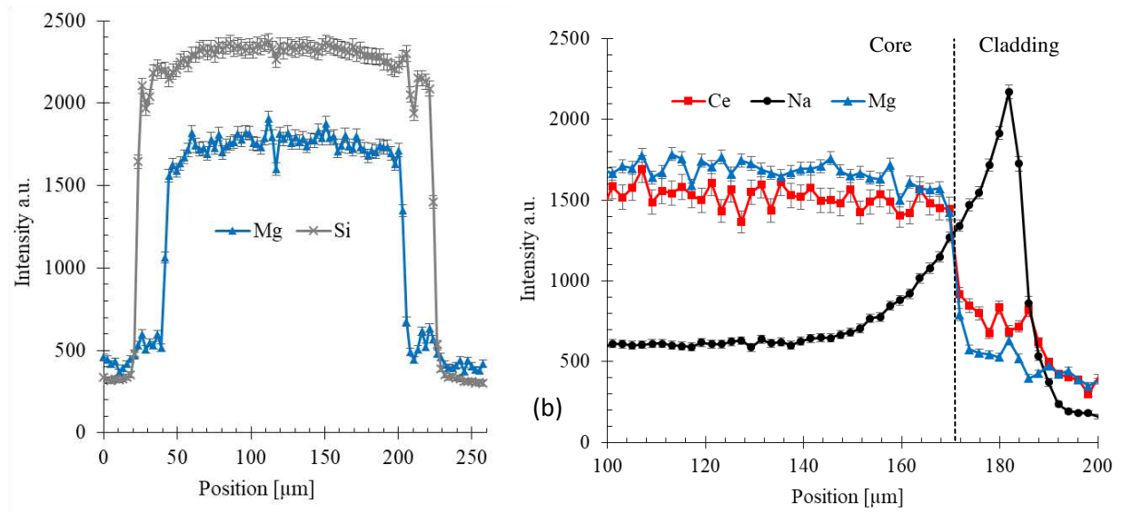
Figure 4. (a) EDS line scan across the entire cane where the core (Mg) and core/cladding (Si) components can be seen, and (b) spectra of the core-cladding interface for Mg, Ce, and Na.
