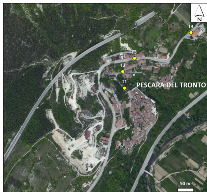
Figure 5.31. Locations of representative noise measurements carried out in the village.
