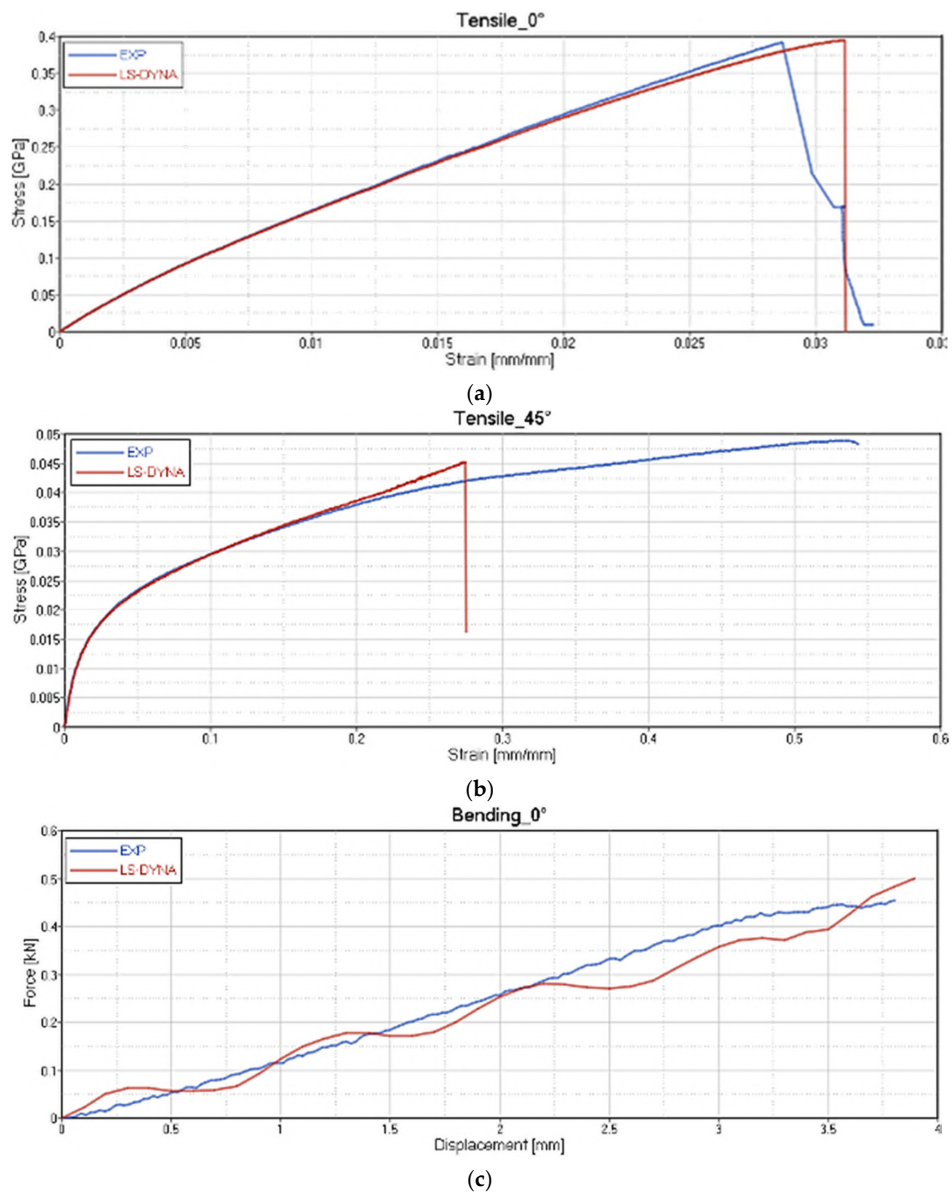
Figure 20. Correlation between experimental data and virtual material card setting for GF/PP. Tensile test at 0° (a); Tensile test at 45° (b) and Force-Displacement (kN-mm) for Bending test at 0° (c).
