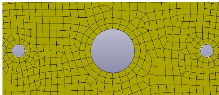
Figure 16. Particular of the model with the constrains on the internal edge of the support pin holes.
