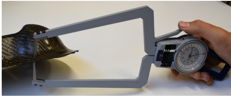
Figure 12. Experimental measurement of wall thickness for GF/PP Double Dome.
