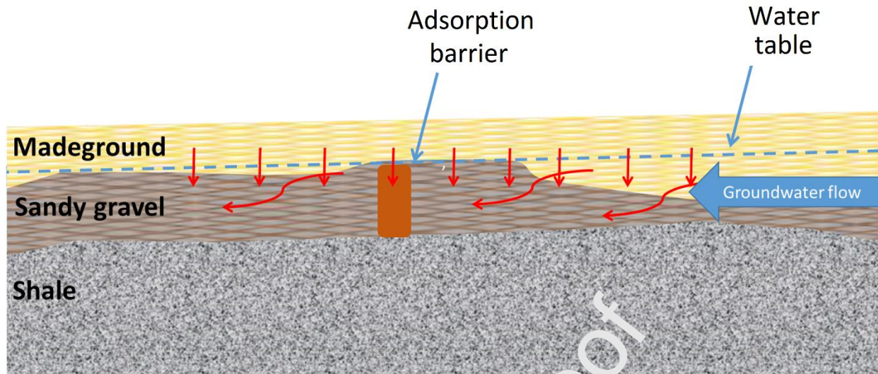
Figure 1. Conceptual model of the Nistratur site in Northern Spain. The red arrows show the passage of heavy metal.
