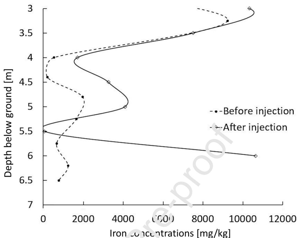
Figure 4: Comparison of the iron content in the sediment before (core taken at IW5, Figure 2a) and after injection of the nanoparticles (core taken at P12, Figure 2a).
