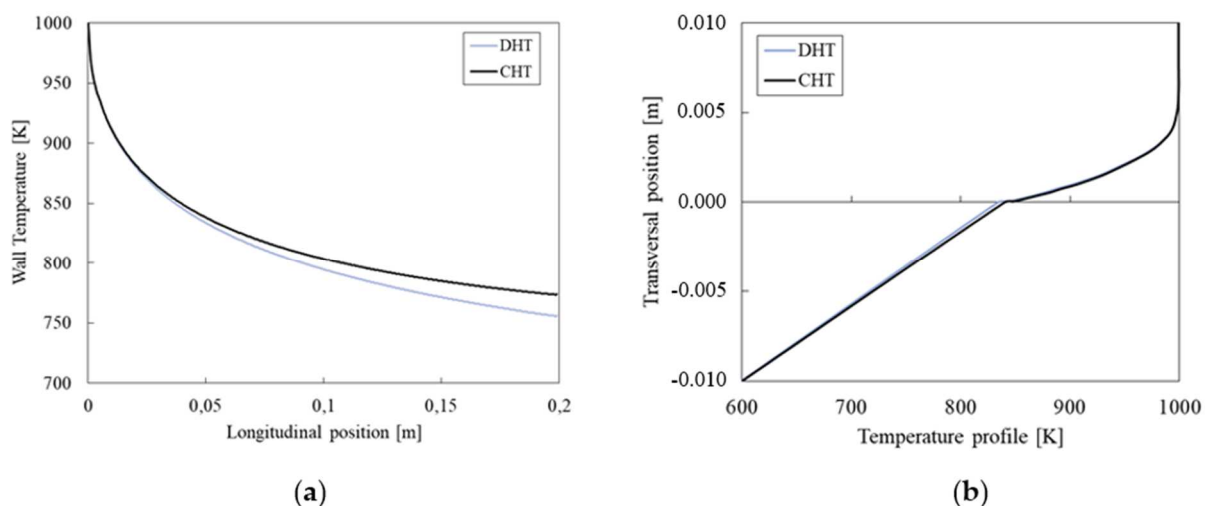
Figure 10. CHT problem for flat plate: (a) temperature at the domain interface, (b) temperature profile at x = 0.05\text{ m} . Numerical vs. analytic solution.
