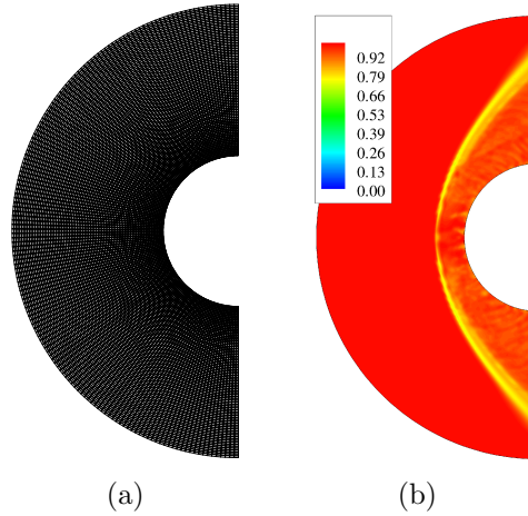
Fig. 4 Computational mesh (a) and element-averaged \theta field (b) for supersonic flow around a circular cylinder
