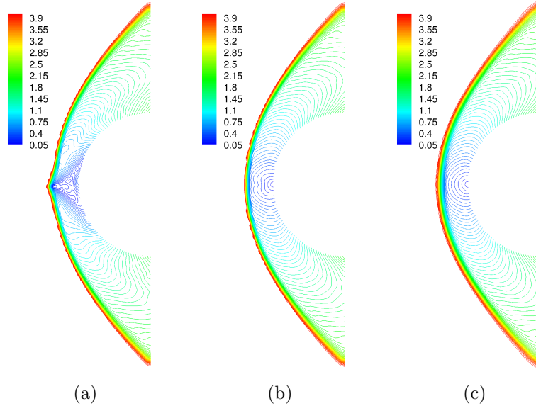
Fig. 5 Mach field around a cylinder at M_\infty = 4 : (a) FDS flux, (b) proposed hybrid flux, (c) LLF flux
