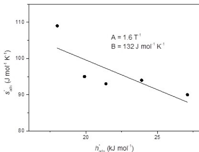
Figure 5. Correlation between entropy and enthalpy of the adsorbed phase ( s_{ads}^* vs. -h_{ads}^* ) for the studied set of CO/zeolite systems.
