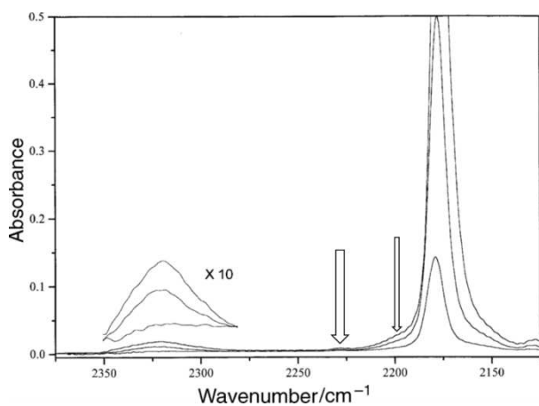
Figure 3. IR spectra of CO adsorbed on Na-ZSM-5. Arrows show combination bands between \nu(\text{C}-\text{O}) and \nu(\text{M}-\text{C}) modes.
