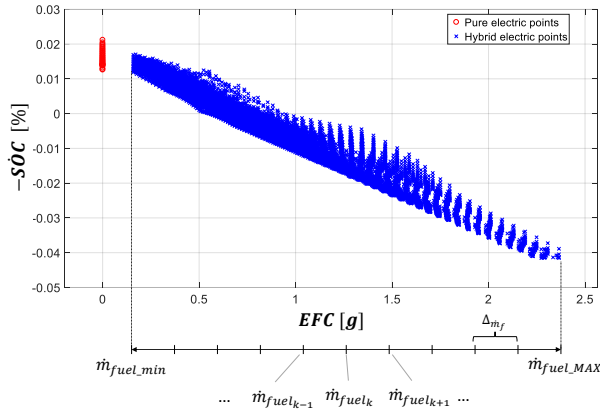
Figure 3. Example of sub-solutions comparison for a sub-problem.
