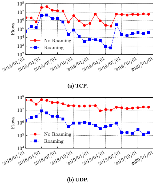
Figure 2: The total number of flows over time for Roaming and Non-Roaming. Notice the log scale on the y-axis.
