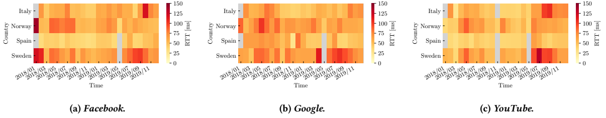
Figure 5: Average RTT.
