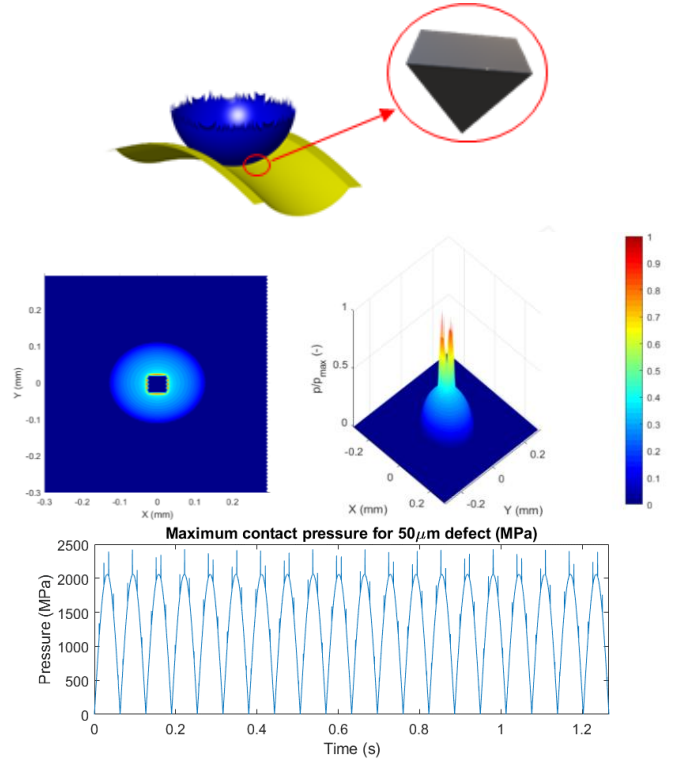
Figure 5. Contact pressure analysis for 50 \mu\text{m} defect.
