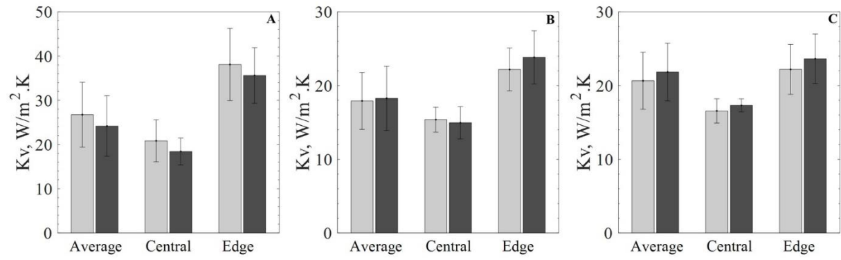
Figure A.4. Mean K_v values. Light grey bars indicate test done without the IR sensor; dark grey bars indicate test done with the IR sensor. (A) Shows results for 4R, (B) for 6R and (C) for 20R vials. Error bars indicate one standard deviation.
