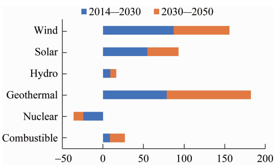
Fig. 6 Projection ratios of EU installed capacities based on WEO 2016 [15]
