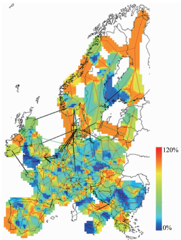
Fig. 11 Power flow distribution for the GEI in 2050
