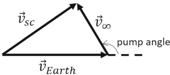
Fig. 5 Pump angle definition diagram
