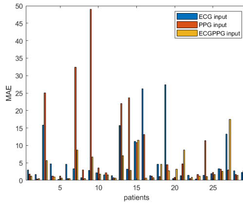
Fig. 8. Mean absolute error for DBP for every patient.
