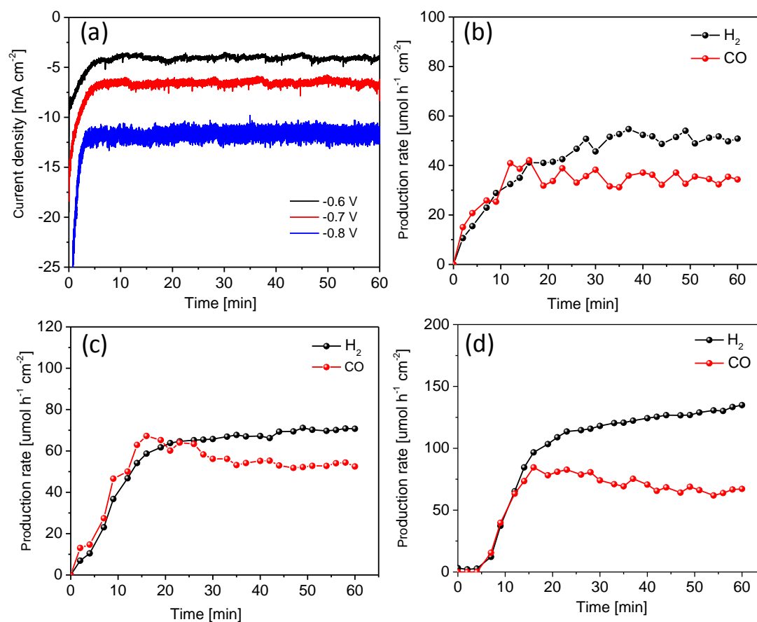
Fig. S6 CA measurements on the Cu-3 electrode in \text{CO}_2 -saturated 0.1 M \text{KHCO}_3 aqueous solutions at various potentials (a). The production rates of \text{H}_2 and \text{CO} at various potentials: -0.6 V (b); -0.7 V (c); -0.8 V (d)
