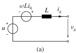
Fig. 3. Equivalent circuits representing the system state-space equations: (a) d -axis current, (b) q -axis current, (c) DC-link voltage and (d) mid-point voltage.
