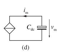
Fig. 3. Equivalent circuits representing the system state-space equations: (a) d -axis current, (b) q -axis current, (c) DC-link voltage and (d) mid-point voltage.
