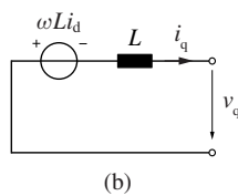
Fig. 3. Equivalent circuits representing the system state-space equations: (a) d -axis current, (b) q -axis current, (c) DC-link voltage and (d) mid-point voltage.
