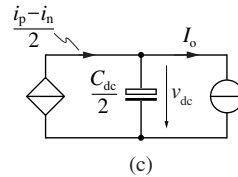
Fig. 3. Equivalent circuits representing the system state-space equations: (a) d -axis current, (b) q -axis current, (c) DC-link voltage and (d) mid-point voltage.
