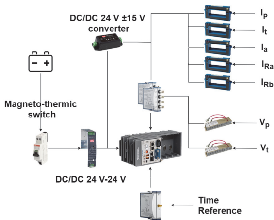
Fig. 4 Measurement setup
