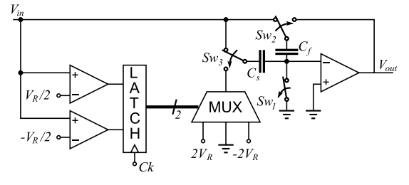
Fig. 4. Schematic of the circuit used for implementing the chaotic map of Figure 3-a.
