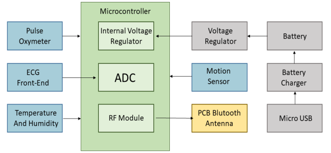
Fig. 2 VITAL-ECG block diagram (device architecture)
